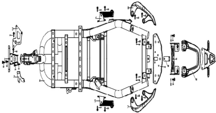
1 Chasis Principal
