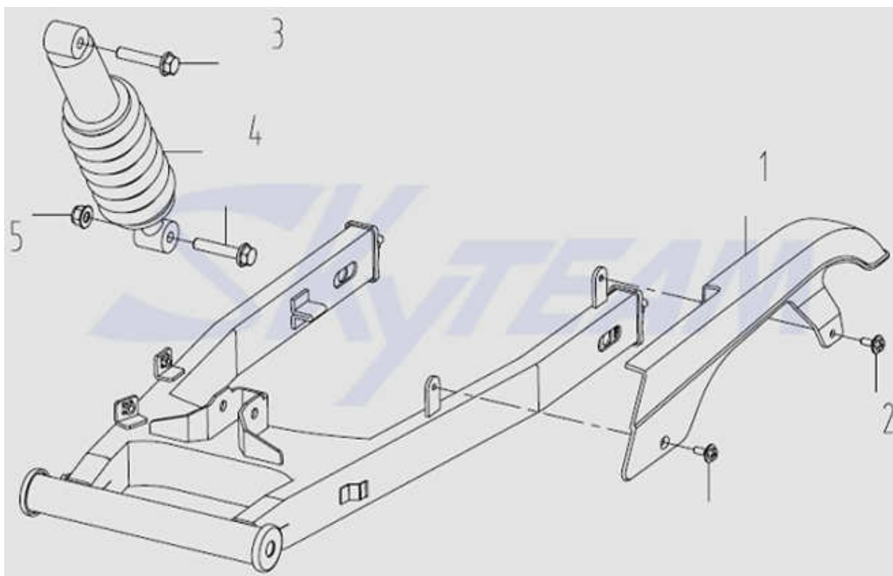
Fig. 6.后减震器 Rear Shock Absorber
