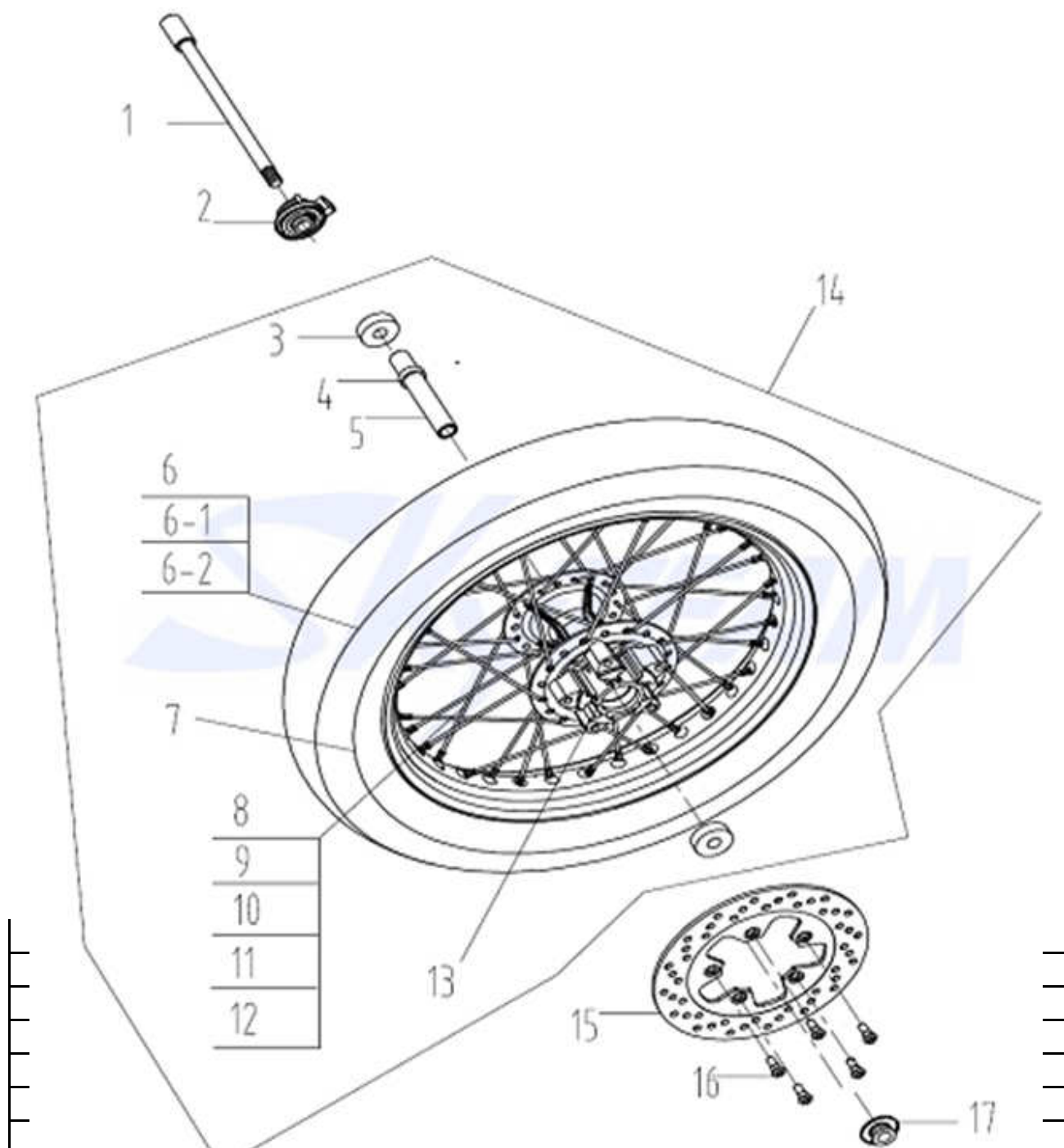
Fig. 5.前轮 Front Wheel
