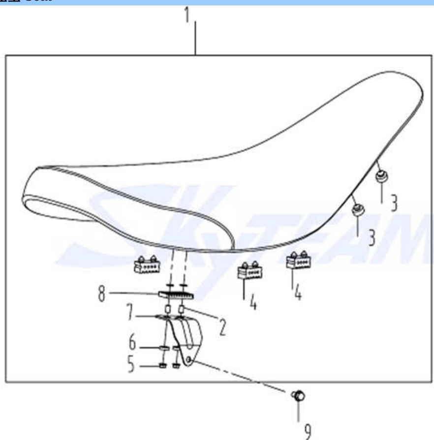
Fig.19.座垫 Seat
