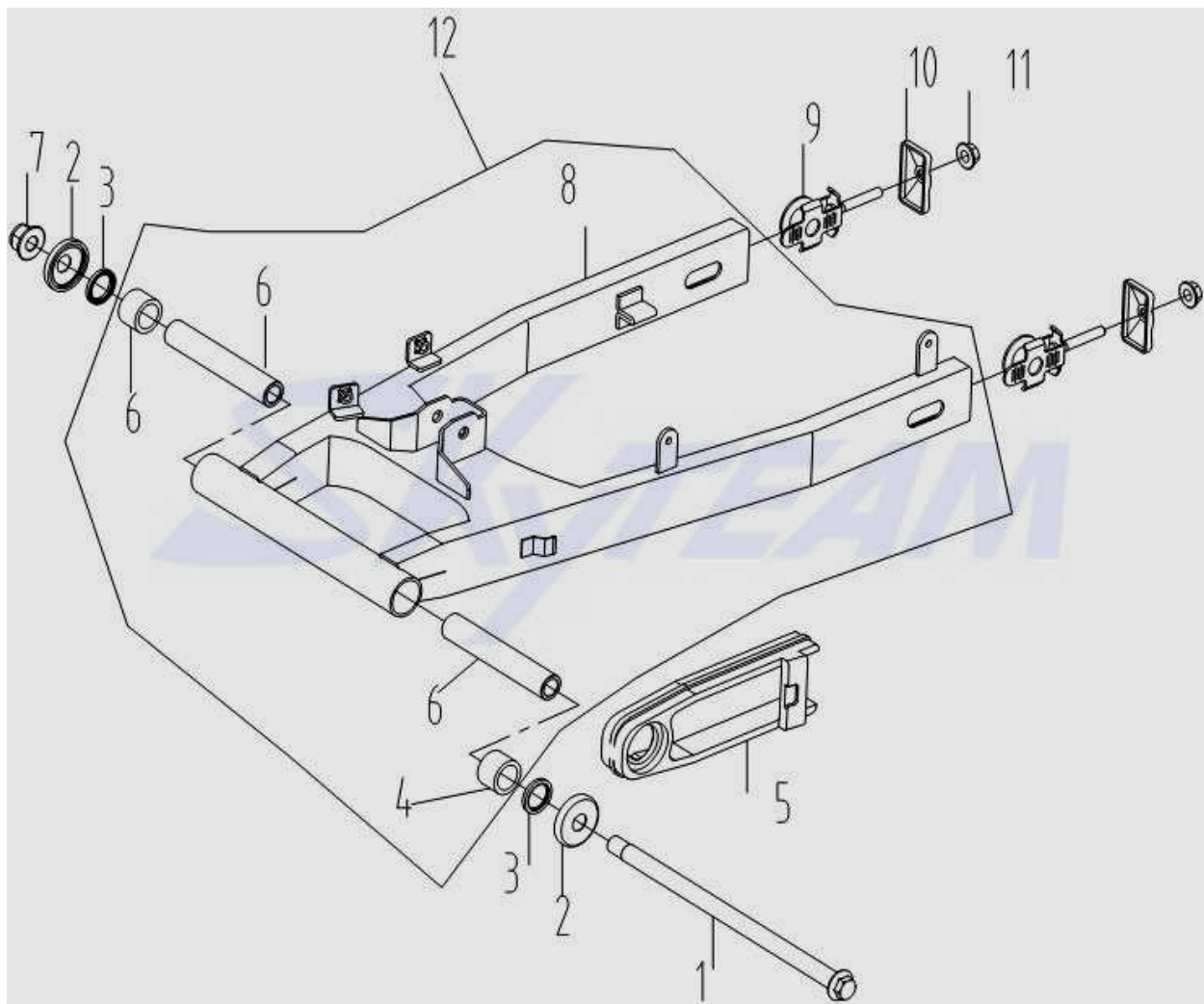
Fig. 9.后摆臂 Rear Swing Arm
