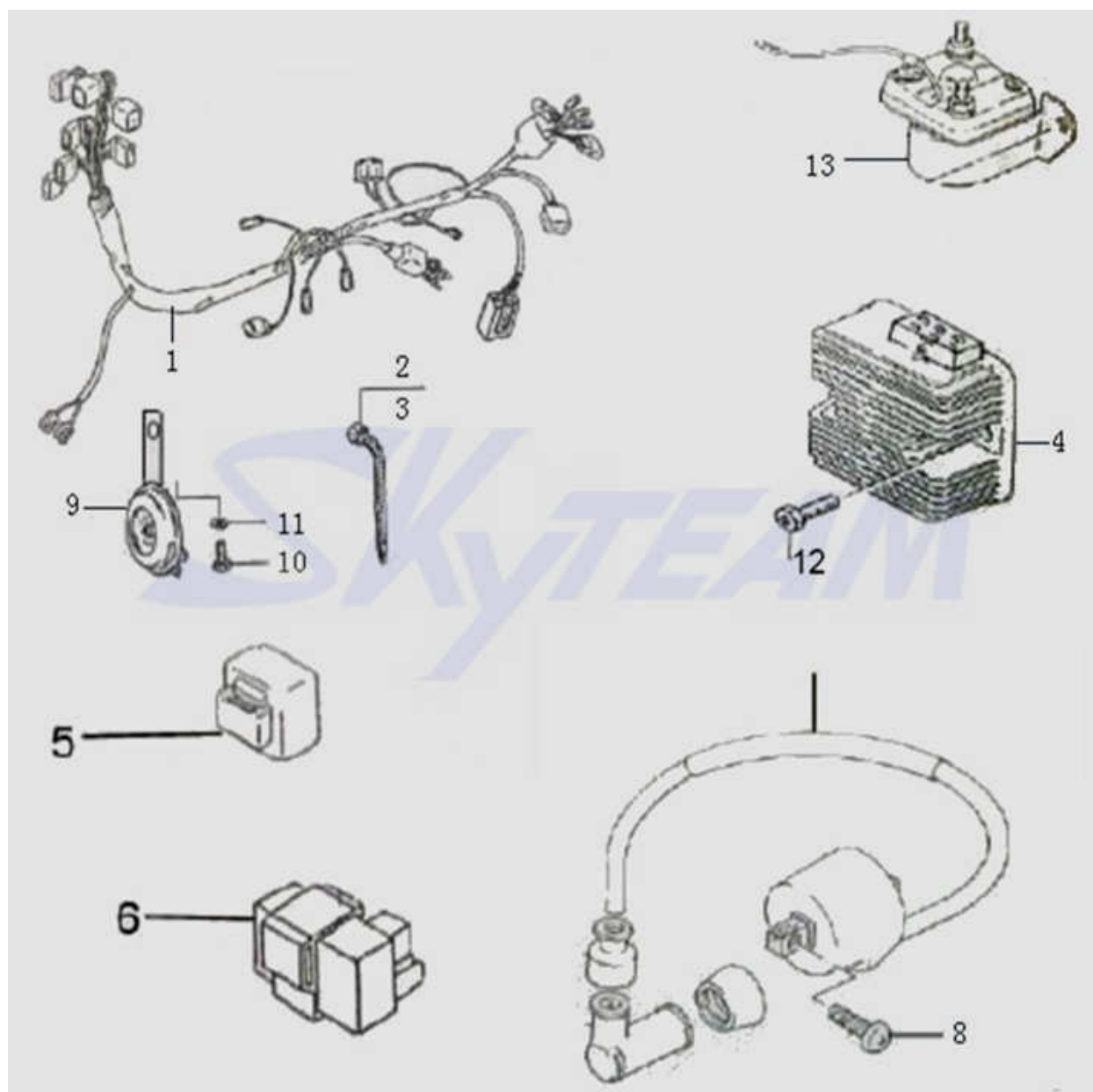
Fig.24. 导线束-电器件Electrical Components
