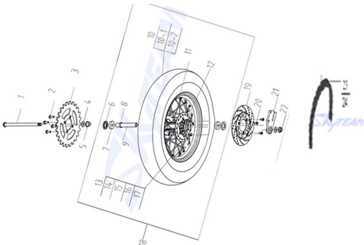
Fig. 8.后轮 Rear Wheel
