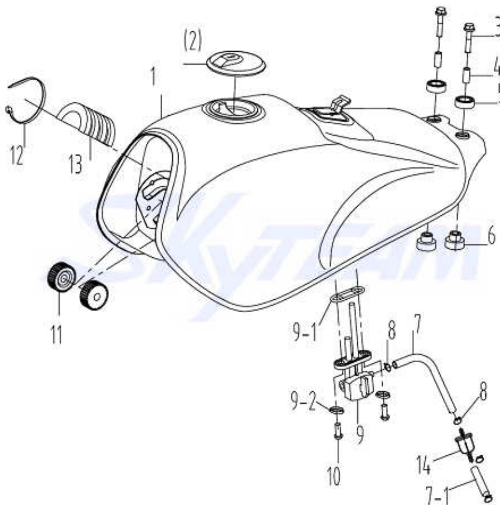
Fig. 2 油箱 Fuel Tank
