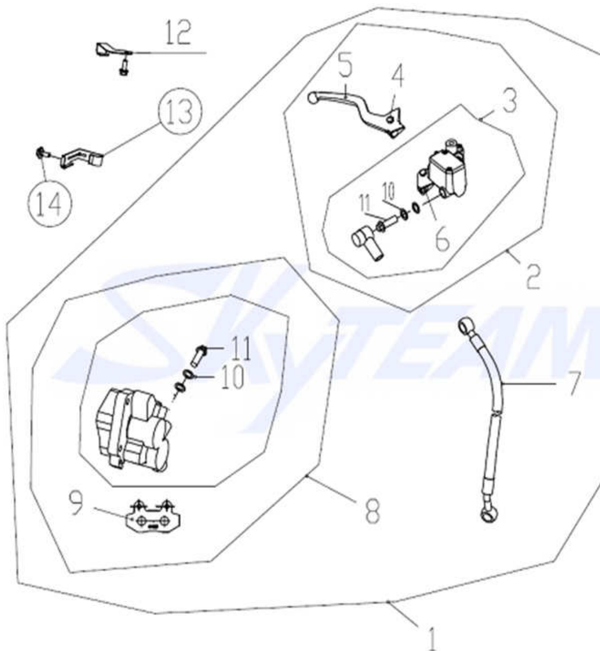
Fig.22.前制动 Front Brake
