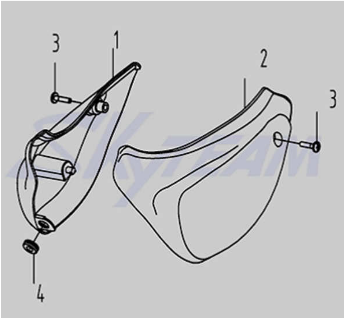
Fig. 13.护板 Side Cover
