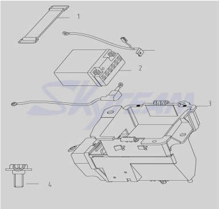
Fig.26. 蓄电池 Battery
