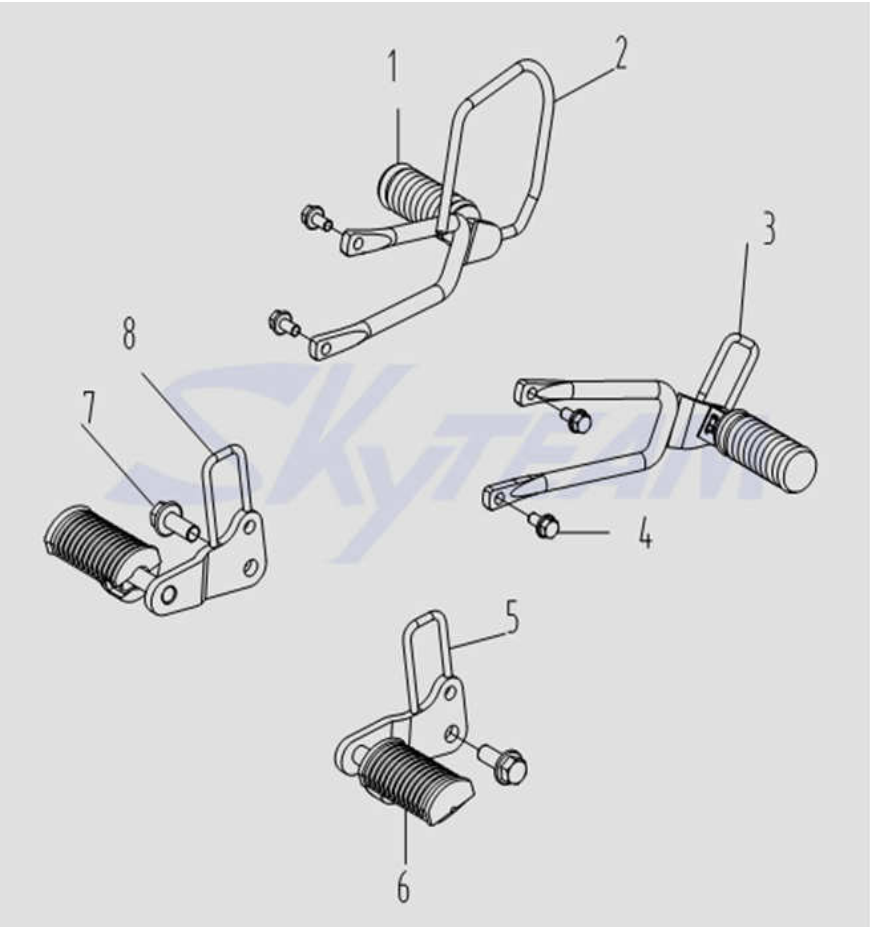
Fig. 7.脚踏Footrest
