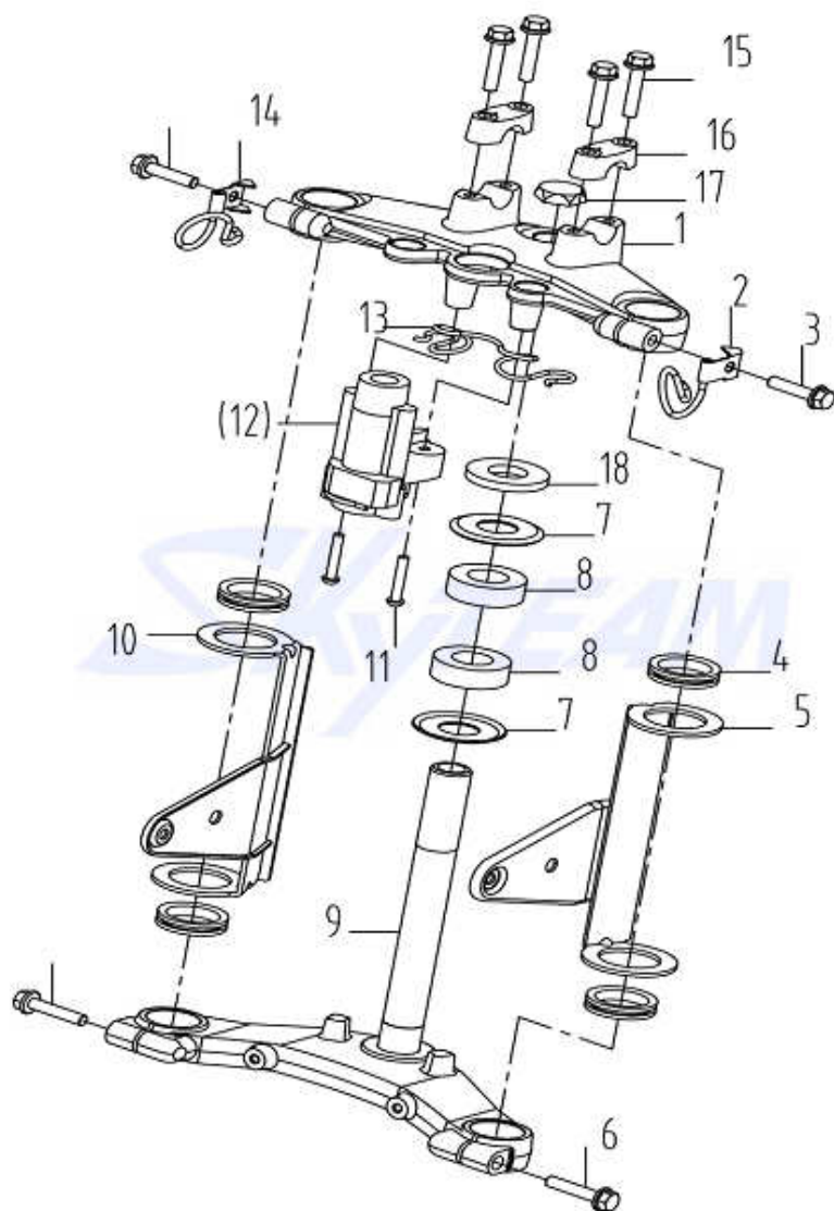
Fig. 4.上下联板 Steering Parts
