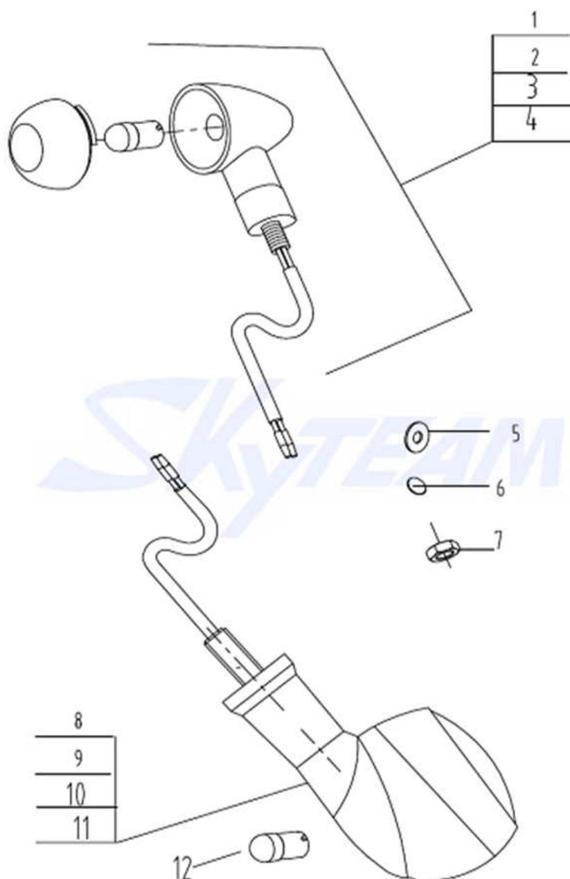
Fig.23.转向灯 Signal Lamp
