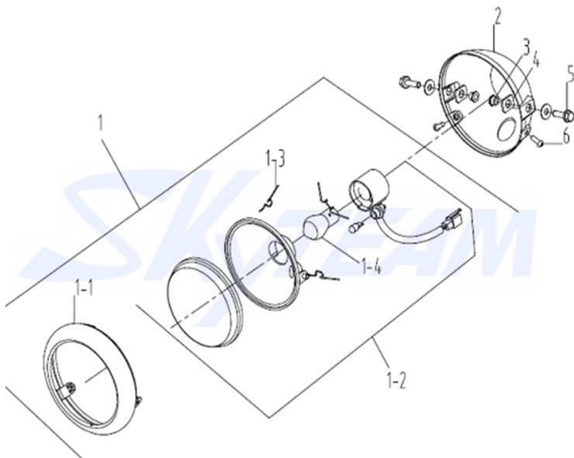
Fig. 17.前大灯 Head Lamp
