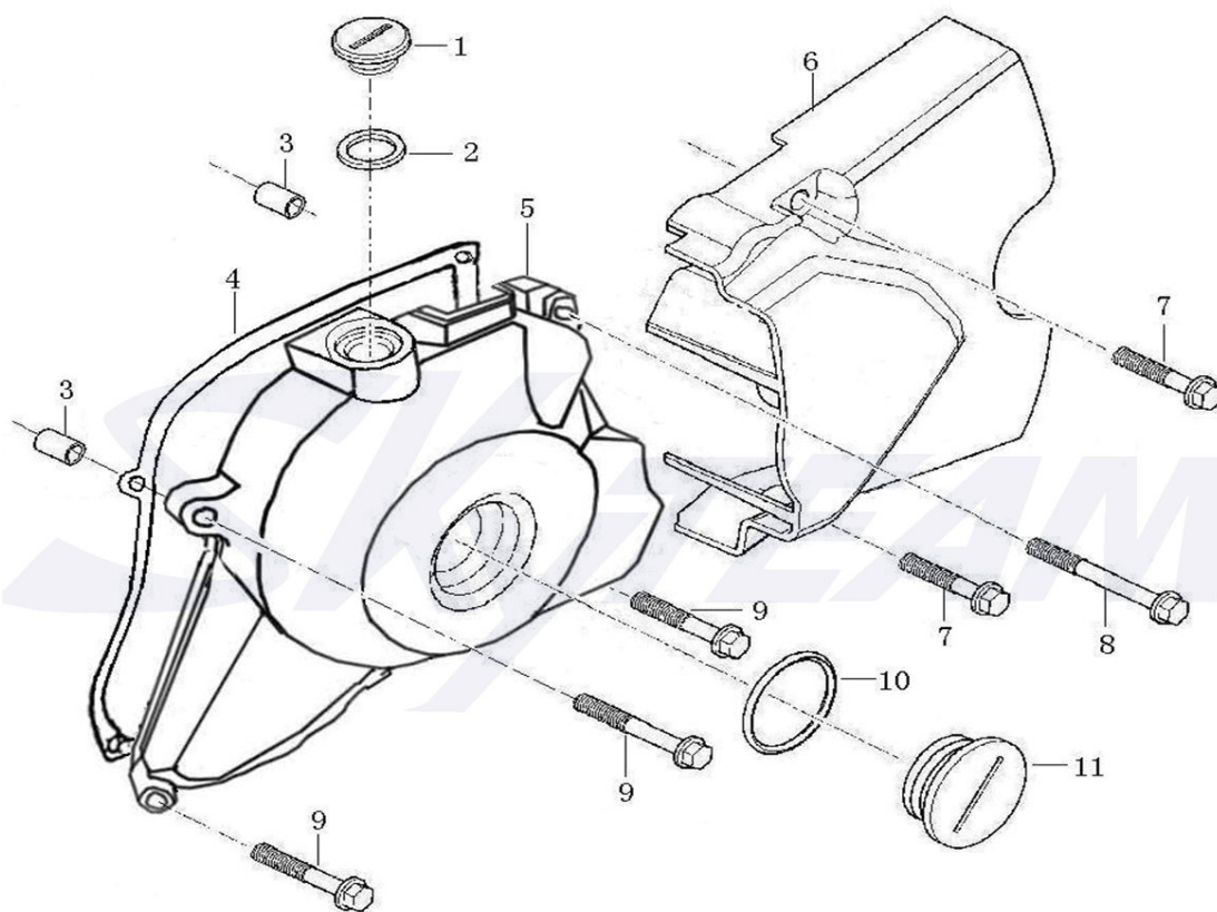
左曲轴箱盖 LEFT CRANKCASE COVER
