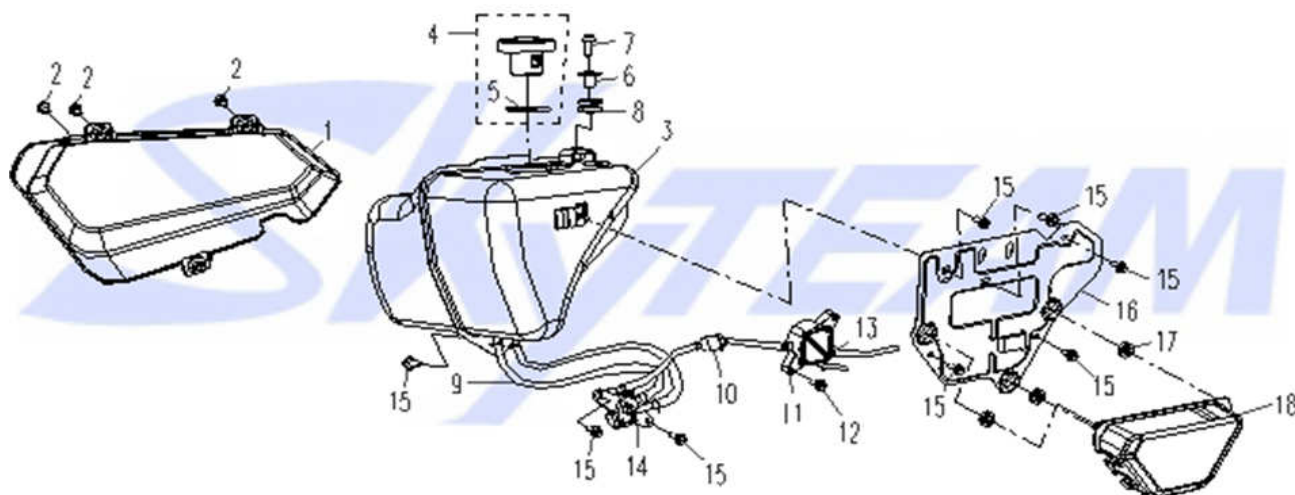
Fig. 7 油箱 FUEL TANK
