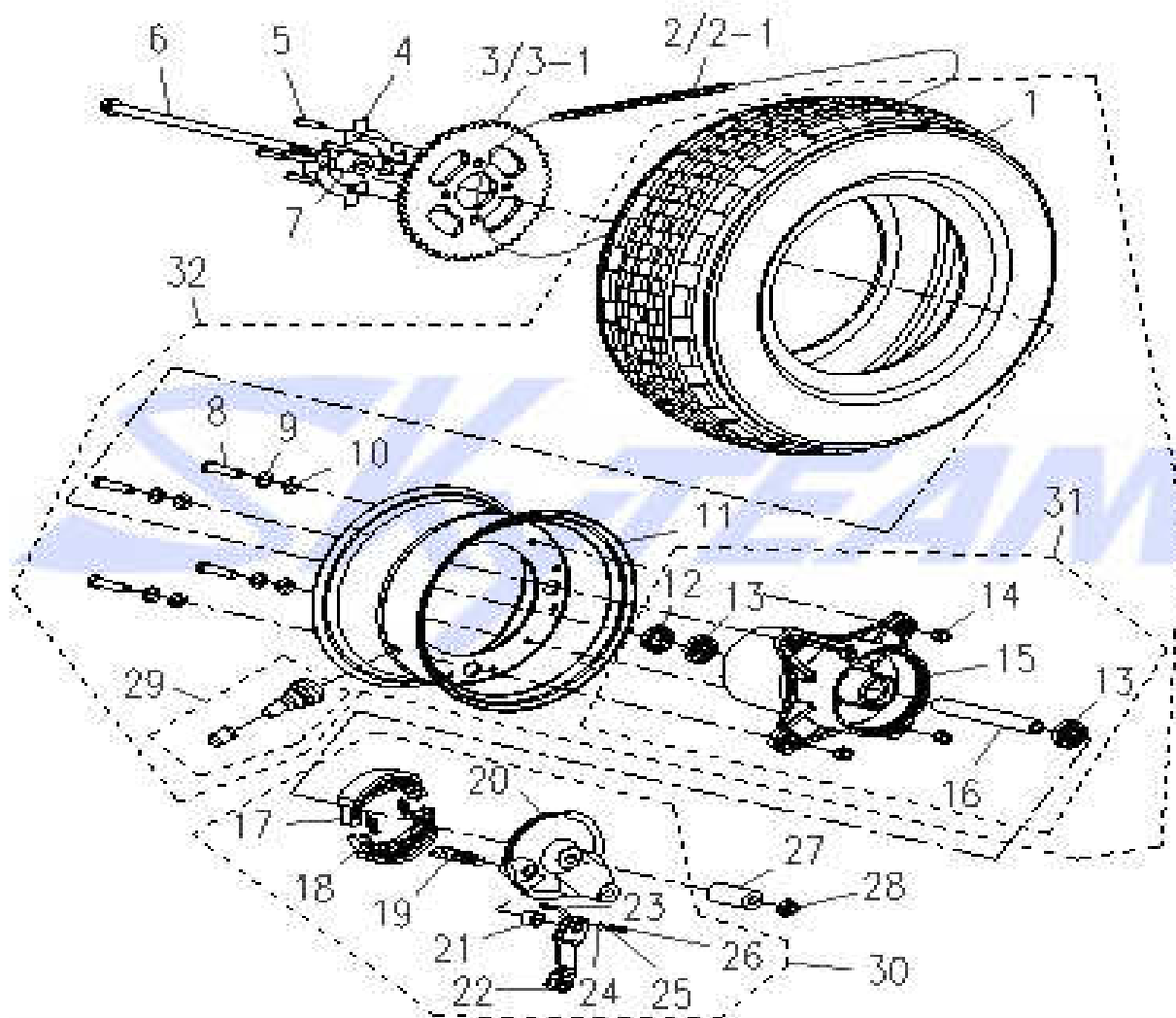
Fig. 13 后轮 REAR WHEEL
