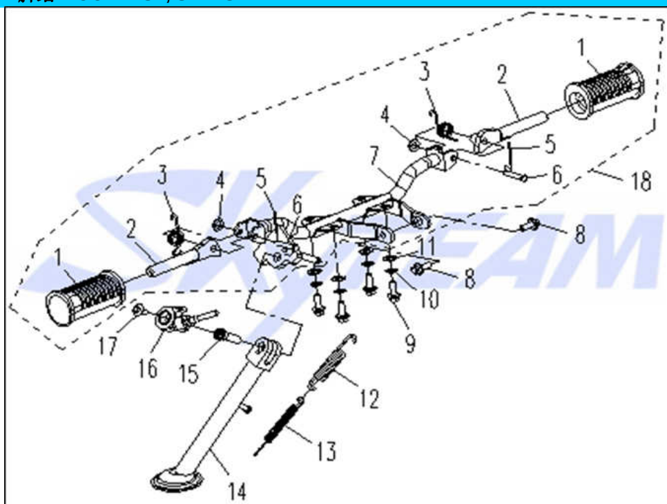
Fig. 9 脚踏 FOOTREST, SIDE STAND
