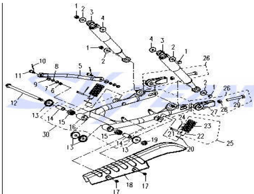
Fig. 14 后悬挂 REAR SUSPENSION
