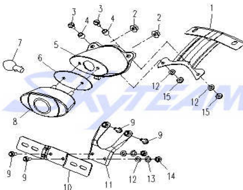
Fig. 3 后尾灯 REAR LAMP
