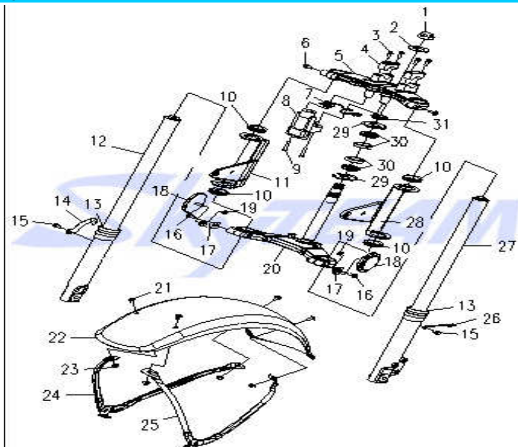
Fig. 11 前悬挂 FRONT SUSPENSION
