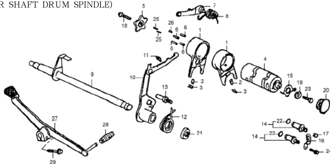
E-14 变速装置 (GEAR SHAFT DRUM SPINDLE)
