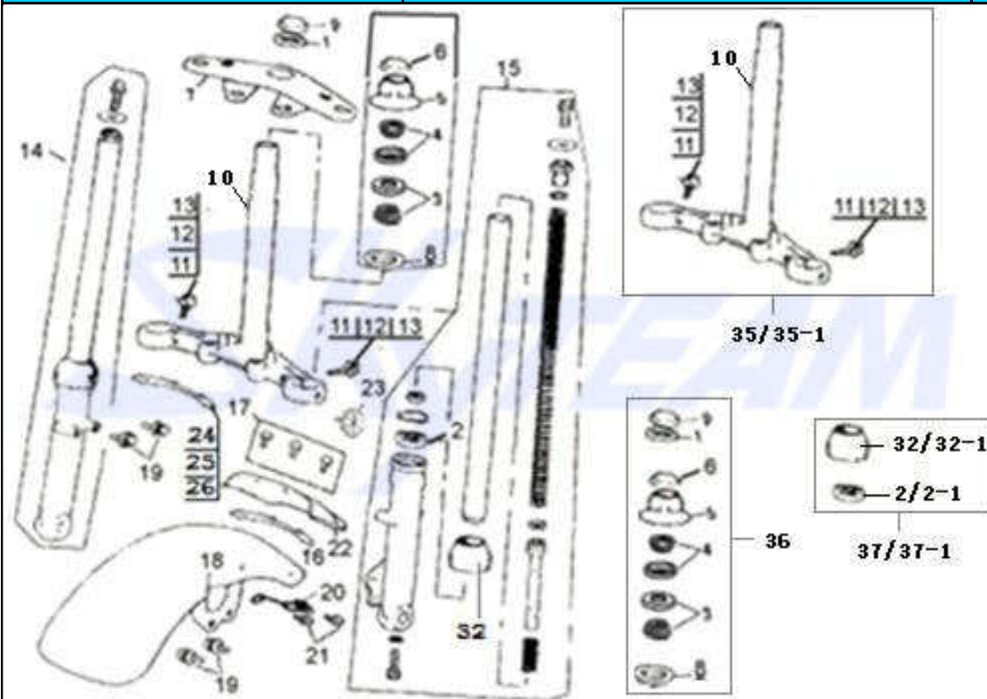
FIG.6 FRONT FORK
