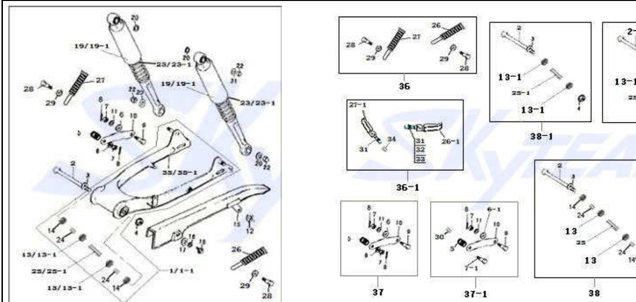
FIG.10 SWINGING ARM & REAR ABSORBER
