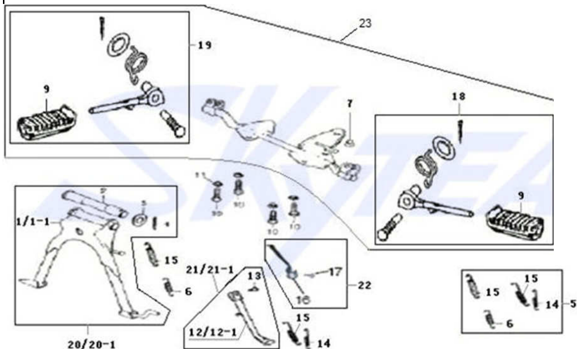
FIG.11 STAND
