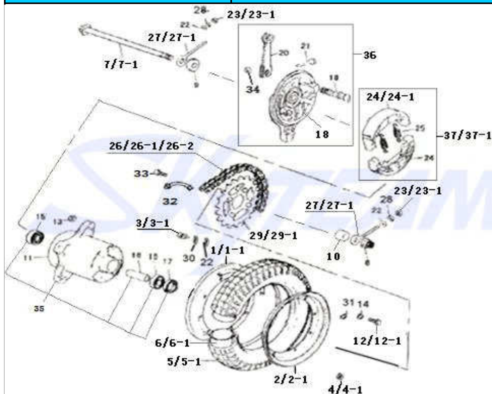
FIG.9 REAR WHEEL
