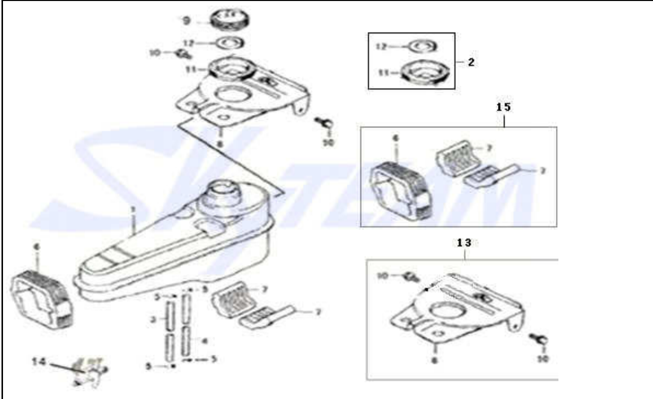
FIG.14 FUEL TANK
