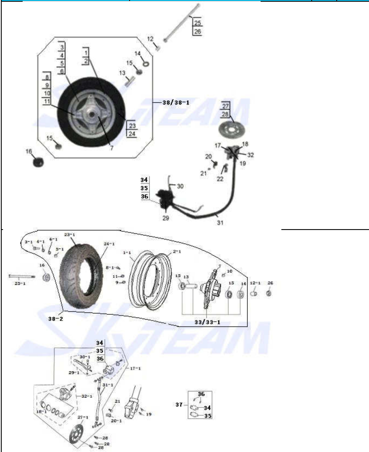
FIG.8 FORNT WHEEL
