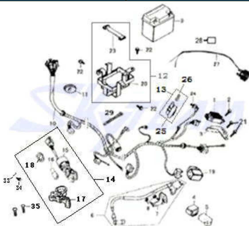
FIG.3 ELECTRICAL
