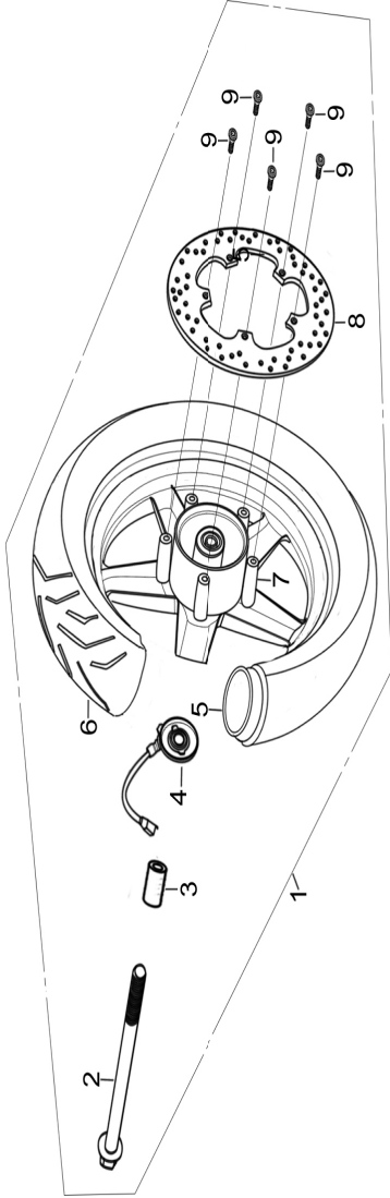
F-10 前轮总成 FRONT WHEEL ASSY
